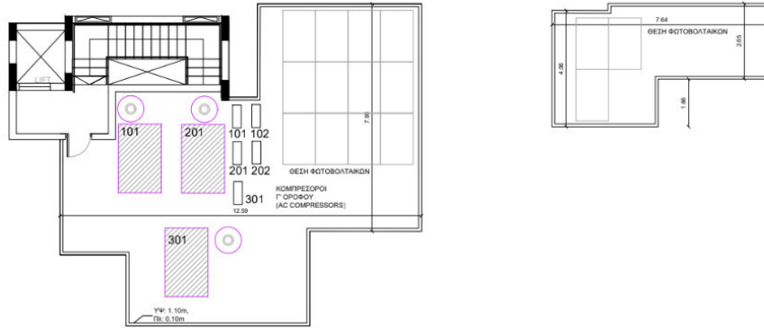
ROOF PLAN VIEW
