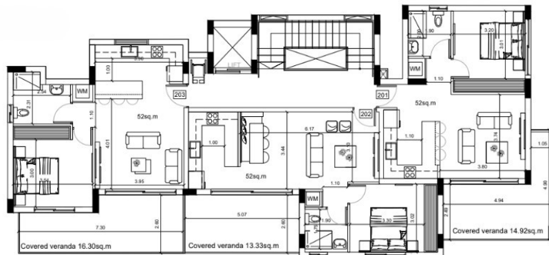
B' FLOOR PLAN VIEW
