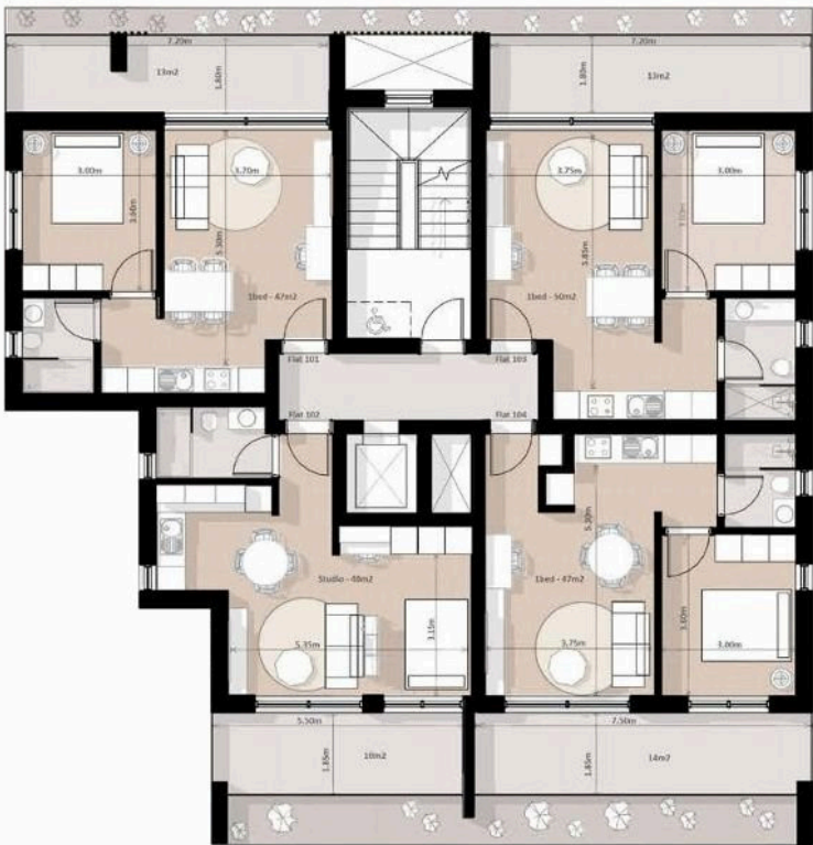
TYPICAL FLOOR
