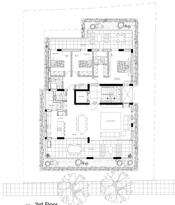
⑤ 3rd Floor 1 : 100
