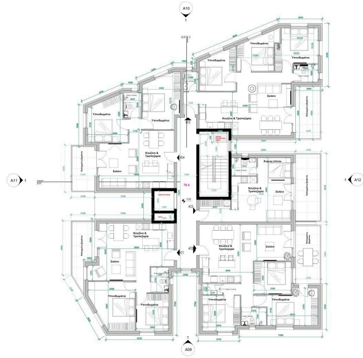
Level 4 1:100
