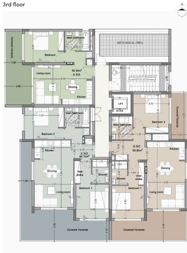
3rd floor
