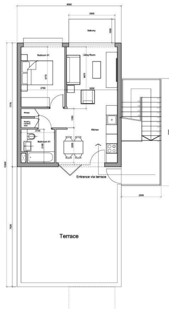
01 1 Bed Cluster - Level 02 Plan 1:50
