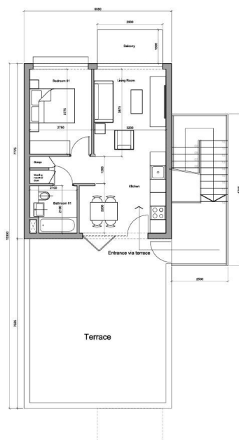
01 1 Bed Cluster - Level 02 Plan
