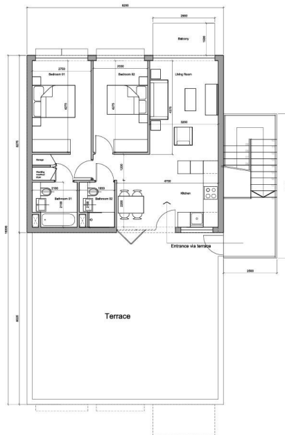
01 2 Bed Cluster - Level 02 Plan
