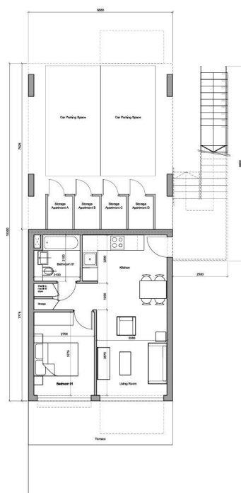
01 1 Bed Cluster - Ground Floor Plan
