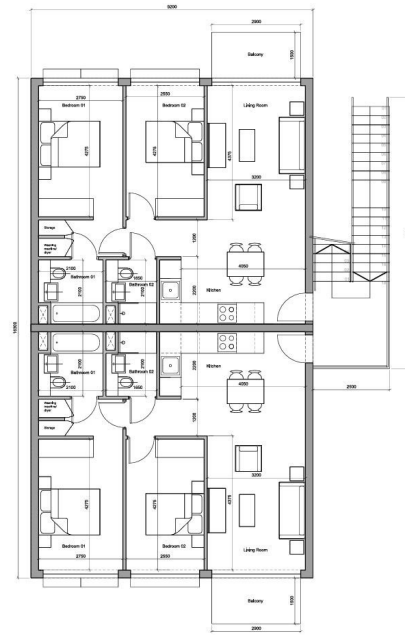
02 2 Bed Cluster - Level 01 Plan
