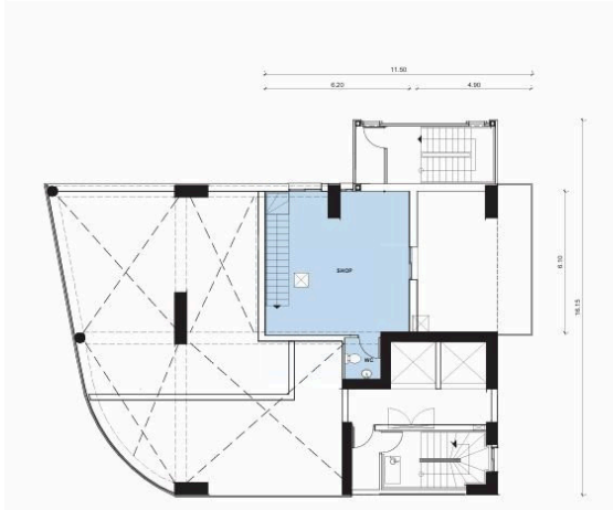
MIDDLE FLOOR PLAN SCALE 1:100
