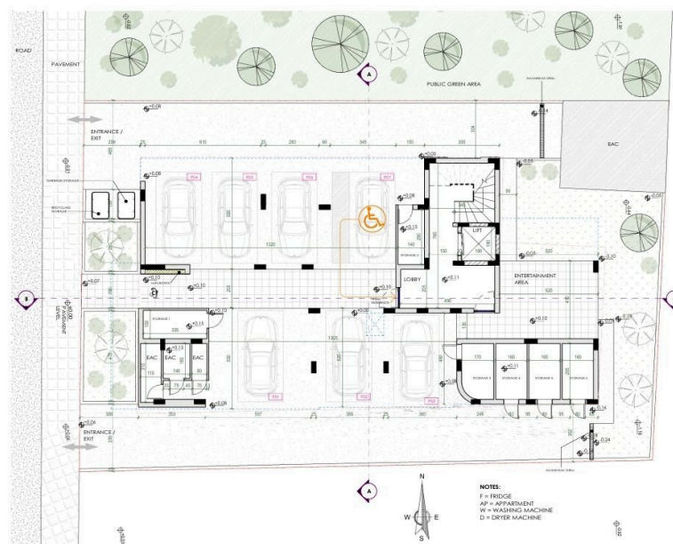
GROUND FLOOR PLAN 1:200
