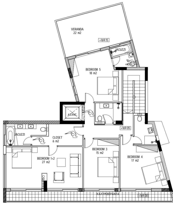
FIRST FLOOR Total area 185 sq.m.
